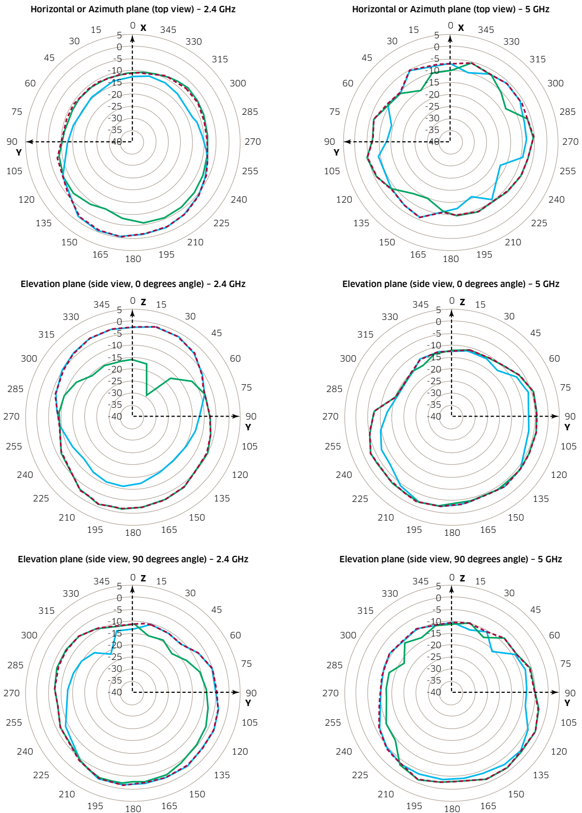
Figure 2. OmniAccess AP1201 antenna pattern plots
